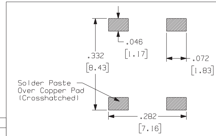
Recommended Solder Pad Geometry
