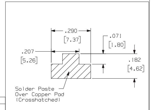
Recommended Solder Pad Geometry
