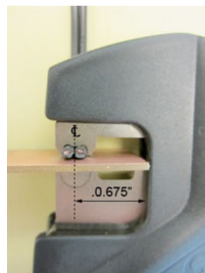
Wire Crimped in Hand Termination Tool
